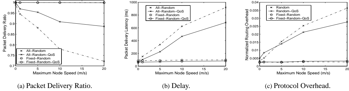
Figure 10. Average quality of flows with 5 sessions in a 250 node network.
