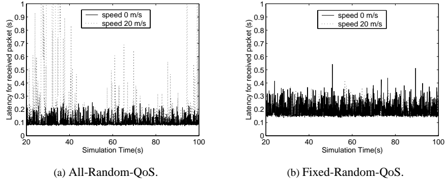
Figure 12. Sample Latency Traces for 250 node networks.
