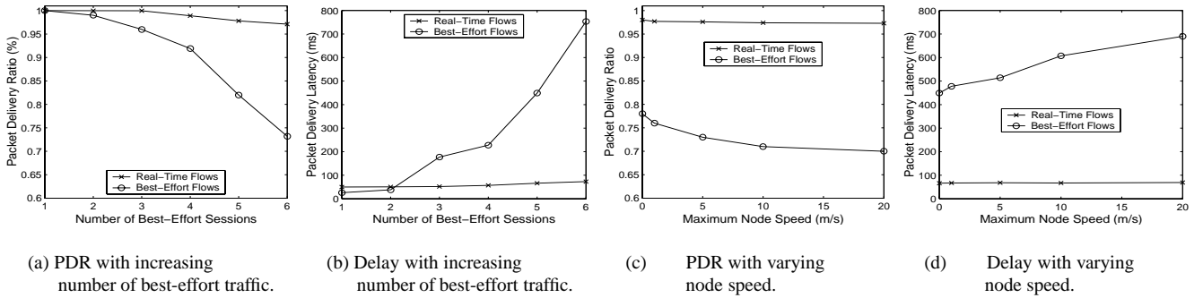
Figure 13. Results for mixed traffic in a 100 node network.
